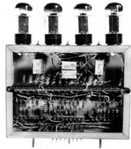
Fig. 6.8. The logic unit of EDVAC
