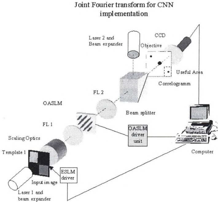
Figure 1. The experimental setup for JTC–CNN implementation measurements.
