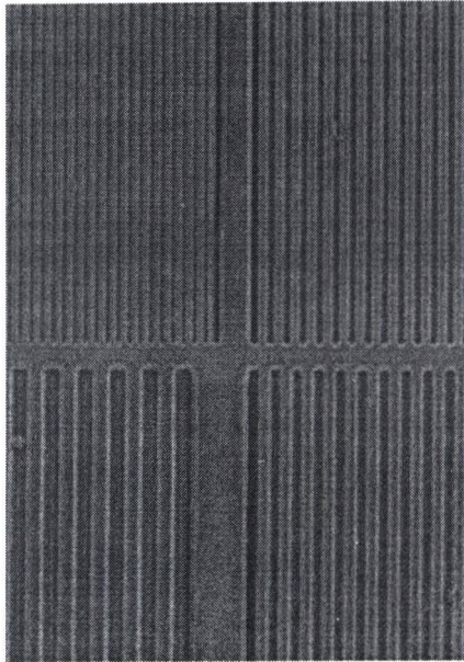
Figure 22. Phase contrast photomicrograph of a grating with no immersion
