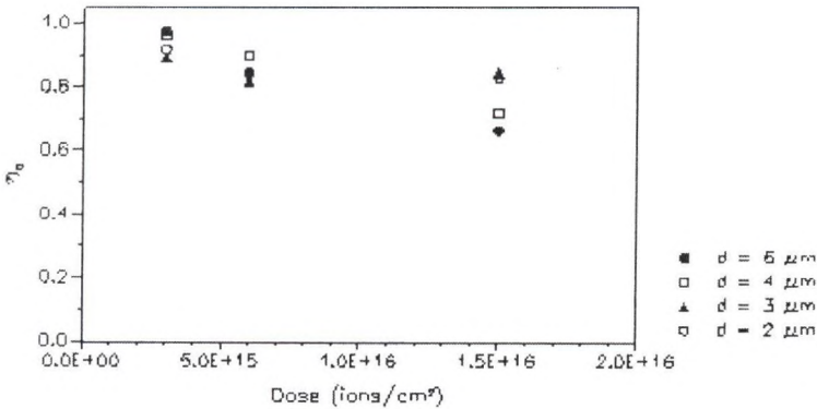
Figure 6. Zero order diffraction efficiency of gratings fabricated by multiple energy implantation of N ions in glass vs. the total implanted dose. E = 500, 800 and 1160 keV.
