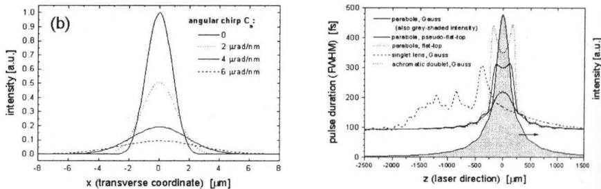
Figure 4: Behaviour of an angularly chirped pulse in the focal area. A Gaussian beam ( d_{FWHM} = 2\text{cm} , truncated to a diameter of d_{max} = 5\text{ cm} ) with a Gaussian spectrum ( \Delta\lambda_{FWHM} = 10\text{ nm} ) is focused by an f = 10\text{-cm} parabolic mirror. Calculations are for four different angular chirps.
