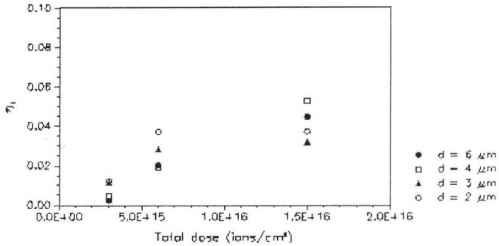
Figure 7. First order diffraction efficiency of gratings fabricated by multiple energy implantation of N ions in glass vs. the total implanted dose. E = 500, 800 and 1160 keV.
