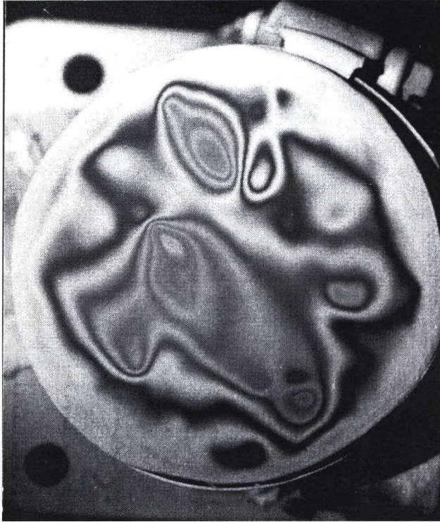
Figure 11. Double-exposed colour hologram of a membrane.
