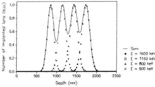
Figure 2. Depth-distribution of the implanted N ions in glass, calculated by TRIM.
