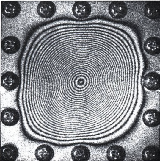
Figure 3. One-picture interferogram of a 8\mu\text{m} central deformation observed through camera lens
