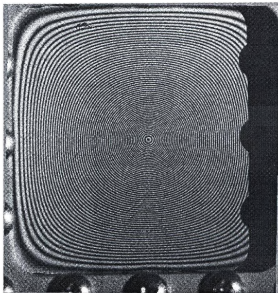
Figure 8. 120-picture composite interferogram of 25 \mu m central deformation /framed fastening/ put together by computer
