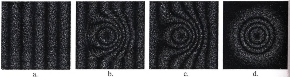
Figure 2. Simulation of difference deformation between simple rotation and deformation. The simulated rotation of the 50x50mm-size object was 0.002 degree, the magnitude of the subtracted deformation was 2\lambda . Correlation fringes of the rotation (a). Difference correlation fringe system using 4 (b), 20 (c) phase shifted reference plane waves. Synthesized correlation fringes of the subtracted deformation pattern using 8 phase shifted reference plane waves (d).
