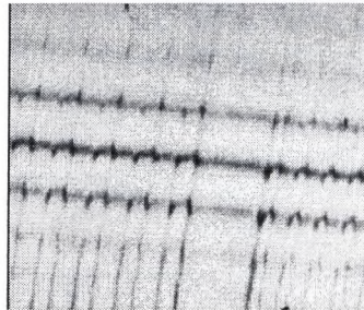
Figure 16. Interferogram of a sample implanted by He ions at E = 800, 650 and 500 \text{ keV} , with a total dose of 1 \times 10^{17} . Gratings with d = 6 and 4 \mu\text{m} .
